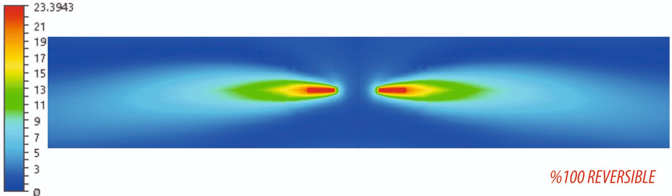
TYPE 400/LR AXIAL JET FAN VELOCITY CHART
